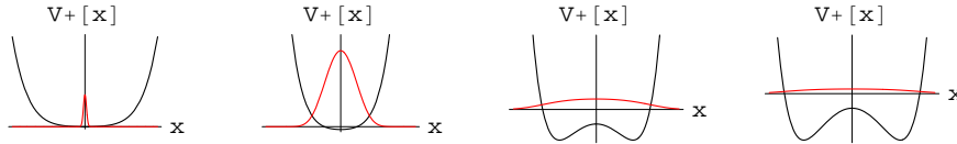
Figure 1.— Potential energy \hat{V}_+ and BPS ground state \Psi_0^G(x) for: (a) \bar{\hbar} = 0.001 , (b) \bar{\hbar} = 0.1 , (c) \bar{\hbar} = 2 , (d) \bar{\hbar} = 4 .
