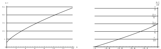
Figure 7.— Mathematica plots of I_1 for \bar{\hbar} = 1 and a > 0 (left) and I_2 for \bar{\hbar} = 0.1 and -1 < a < 0 (right) as function of a . The intersection points with n\pi\bar{\hbar} giving the eigenvalues are also shown.
