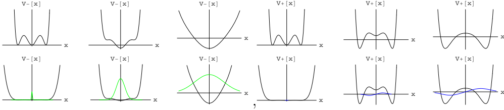
Figure 5.— Potential energy V_\pm(x) and wave function \Psi_\pm^{E_1^\pm}(x) plotted as functions of x for several values of \bar{\hbar} : (a)(a') \bar{\hbar} = 0.001 , (b)(b') \bar{\hbar} = 0.1 , (c)(c') \bar{\hbar} = 1 .
