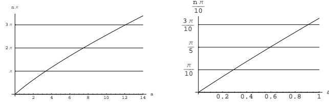
Figure 6.— Mathematica plot of I as a function of a and intersection with n\pi\bar{h} for low n and \bar{h} = 1 (left) and \bar{h} = 0.1 (right)
