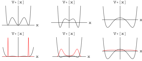
Figure 4.— Potential energy V_+ and BPS wave function \Psi_0^G(x) plotted as functions of x for several values of \bar{\hbar} : (a) \bar{\hbar} = 0.001 , (b) \bar{\hbar} = 0.1 , (c) \bar{\hbar} = 2 .
