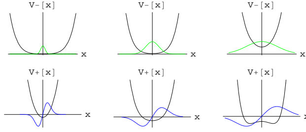
Figure 2.— Potential energies \hat{V}_{\pm} . Degenerate in energy \Psi_{-}^{E_1^{-}}(x) and \Psi_{+}^{E_1^{+}}(x) wave functions: (a) \bar{\hbar} = 0.01 , (b) \bar{\hbar} = 0.1 , (c) \bar{\hbar} = 1 .
