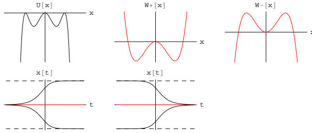
Figure 3.— (a) Potential energy U(x) . (b) Superpotential W^\pm(x) . (c) Zero-energy, finite action, trajectories (instantons).
